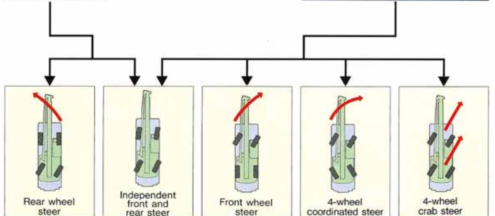
Rear steering control switch
